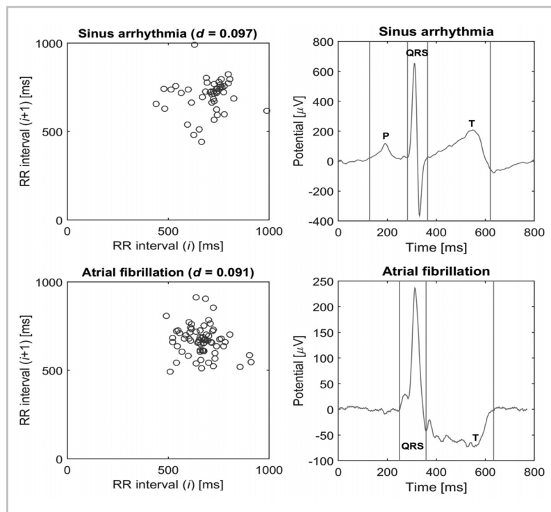
Figure 2. Poincaré plot (on the left) and the corresponding average majority cycle (on the right) with the identified ECG wave limits (vertical red lines) related to sinus arrhythmia and AF. In the case of AF, P wave cannot be seen on the average cycle.
