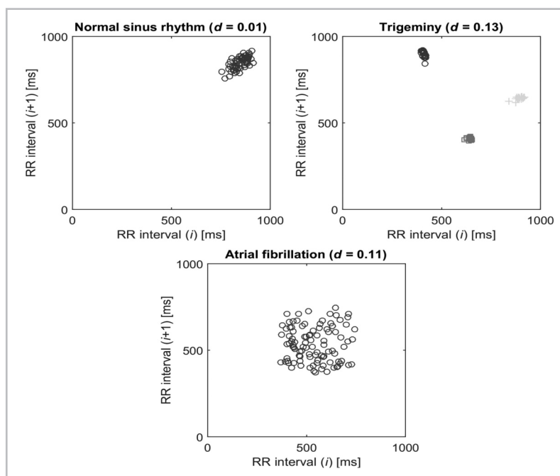
Figure 1. Poincaré plots representing normal, trigeminy (with 3 well-defined clusters) and AF rhythm. Each Poincaré plot belongs to a 1 minute long ECG record with approximately 70 points. The parameter of d is the dispersion along the diagonal.
